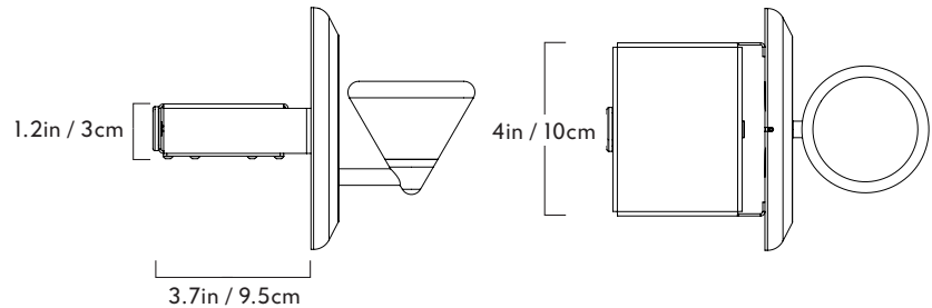
240V Driver Housing
