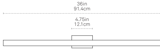
JUNCTION-BOX MOUNTED - Requires Plate -
