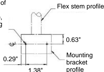
MOUNTING HOLES Dimensions in inches
