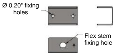
MOUNTING BRACKET Dimensions in inches
