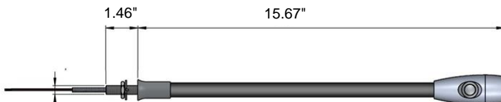
Light Dimensions in inches
