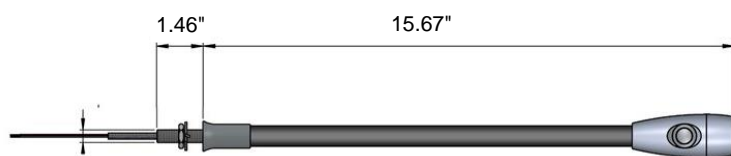
Light Dimensions in inches
