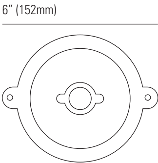
Backplate
