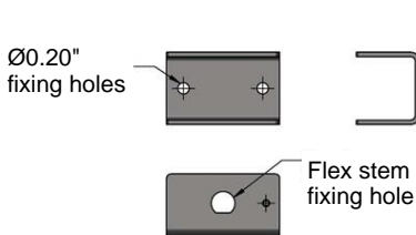
MOUNTING BRACKET Dimensions in inches
