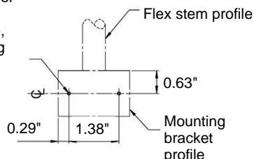
MOUNTING HOLES Dimensions in inches
