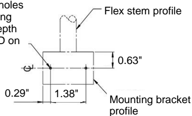
MOUNTING HOLES Dimensions in inches
