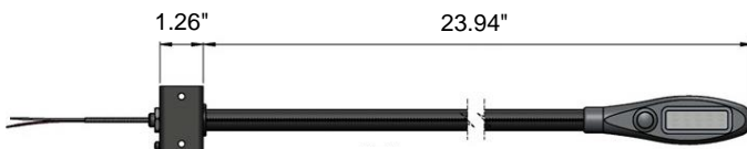
LIGHT Dimensions in inches
