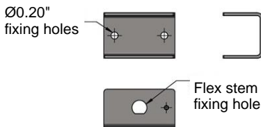
MOUNTING BRACKET Dimensions in inches
