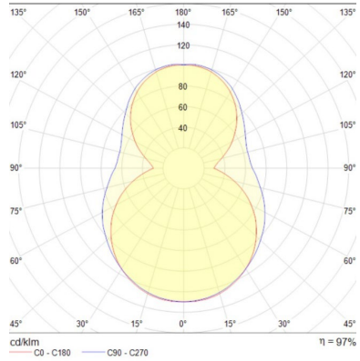
Photometric curve (.ldt and .ies)
